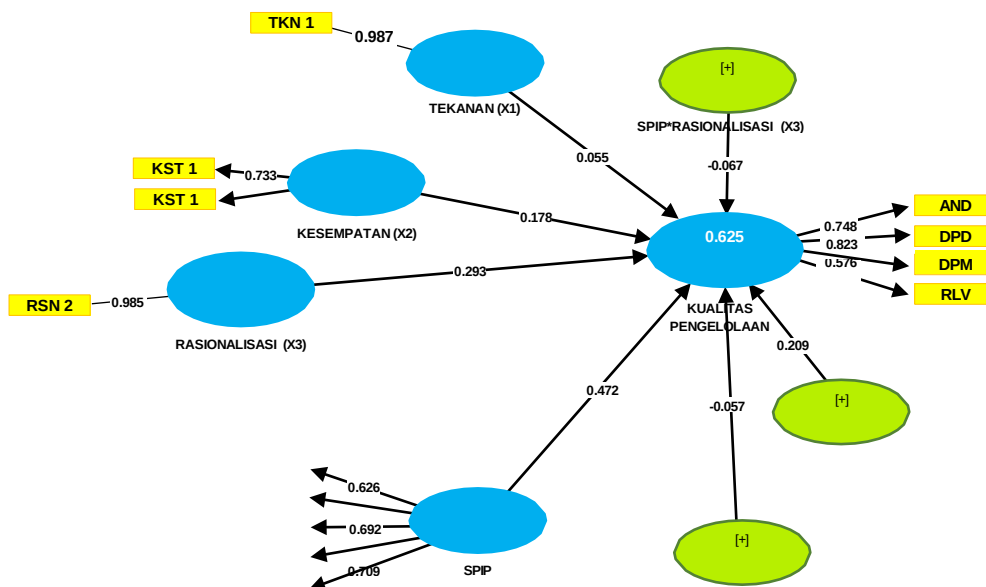
Gambar .3 Model Struktural
